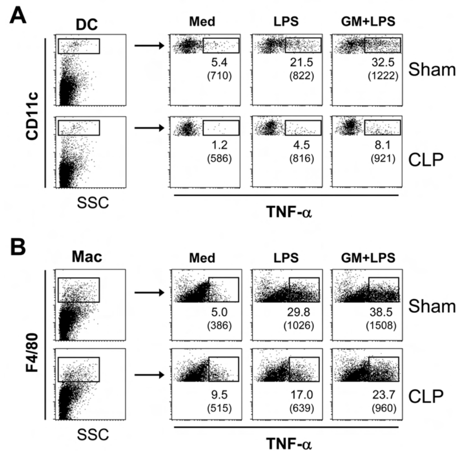
Figure 7. Modulation of the expression of TNF- \alpha through GM-CSF in splenic DC and macrophages. At 24 h after CLP or sham operation ( n = three to four mice per group), total spleen cells were pooled and cultured in medium alone (Med), or were stimulated with LPS or with GM-CSF (GM) + LPS for 8 h. Monensin was present during the last 6 h of culture. After surface staining of CD11c or F4/80, cells were fixed, permeabilized, and stained for intracellular TNF- \alpha . CD11c-positive DC (A) and F4/80-positive macrophages (B) were gated and the percentage of TNF- \alpha -positive cells was determined according to staining with the isotype control antibody. The numbers indicate the percentage of TNF- \alpha -positive cells and the respective mean fluorescence intensity of TNF- \alpha staining (in brackets). Data are representative for two experiments. SSC, side scatter; DC, dendritic cells; Mac, macrophages.
